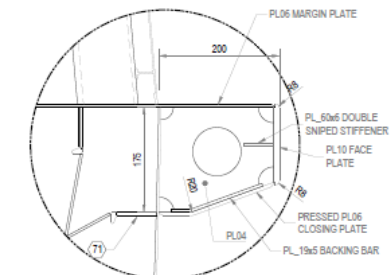
DETAIL 1 - SPONSON
