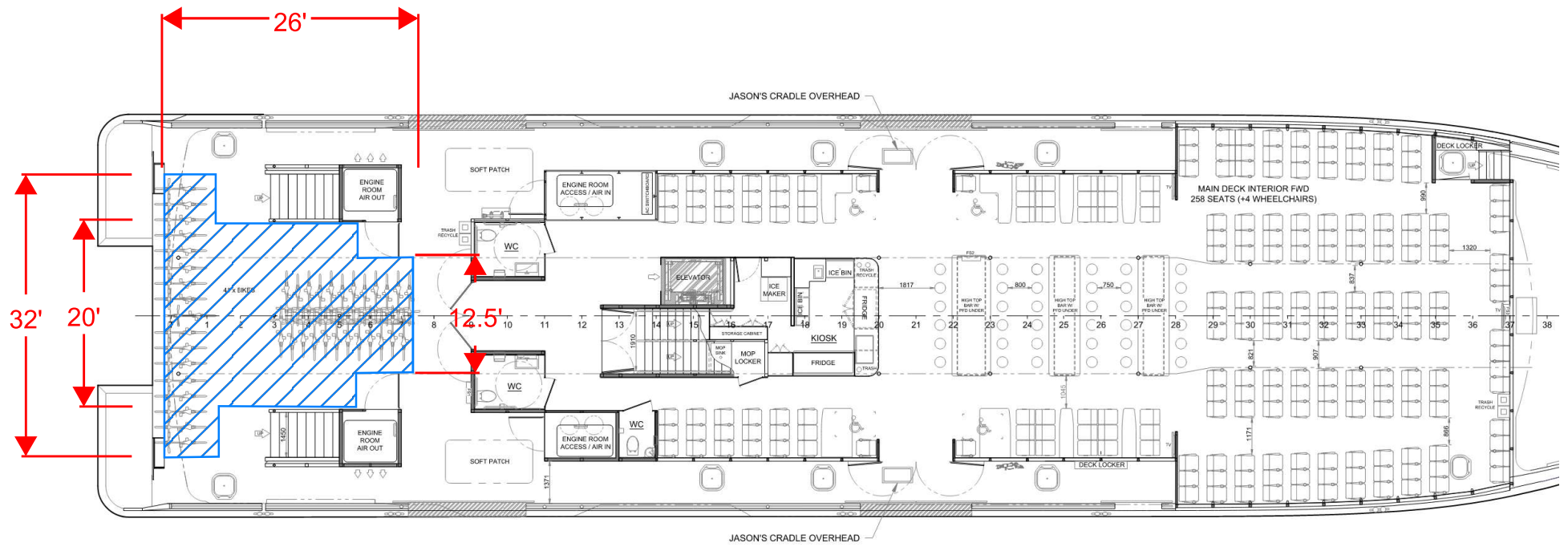
MAIN DECK
