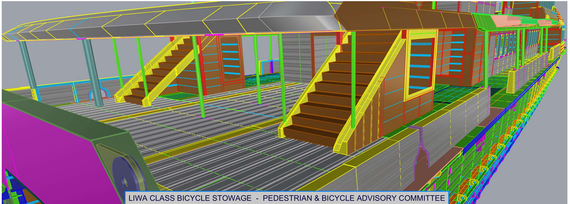
MAIN DECK
