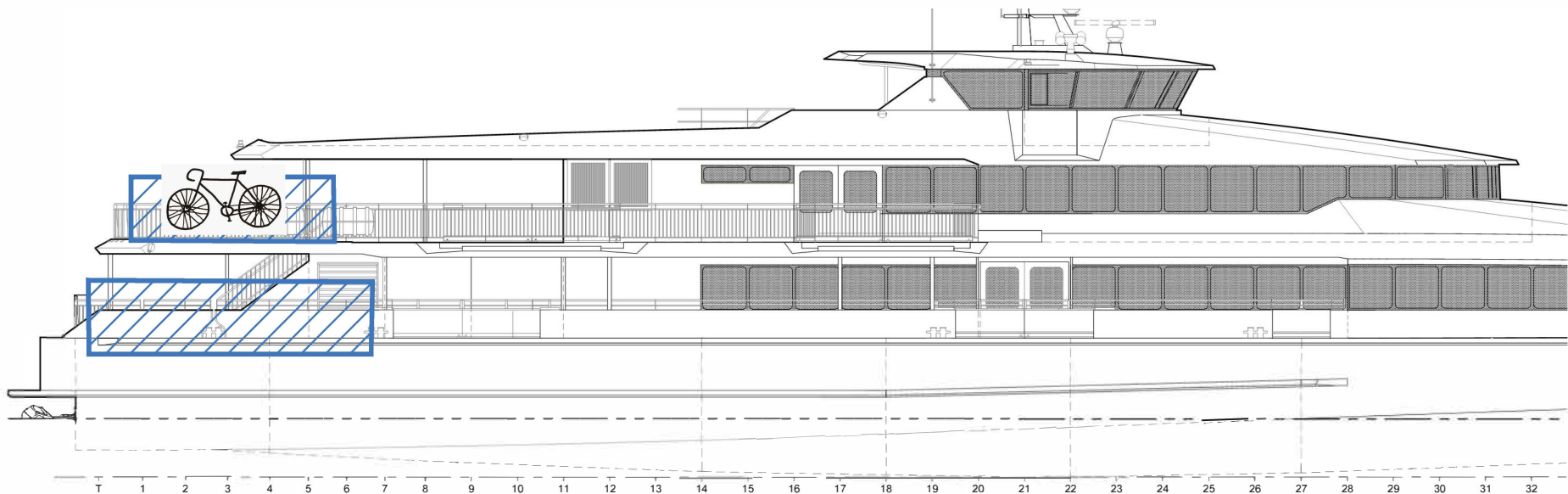
OUTBOARD PROFILE
